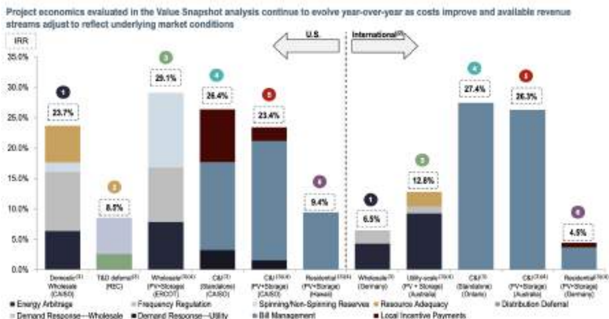
Figure 14. Value Snapshot Case Studies. Taken from Lazard's Levelized Cost of Storage Analysis - Version 7.0
