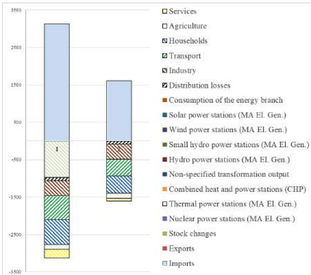
Figure 40. Natural Gas Demand Forecast for 2040, Mm³: 1. Baseline, 2. Accelerated development.
