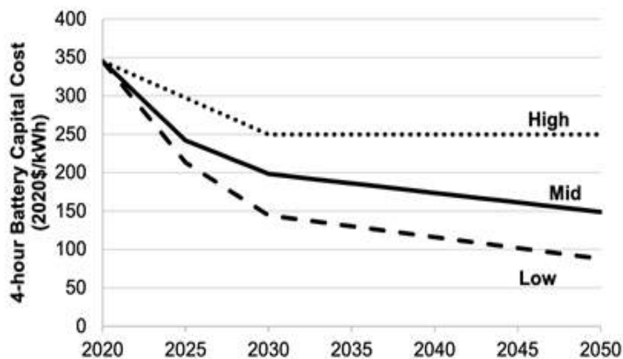
Figure 30. Battery cost projections for 4-hour lithium ion systems.
