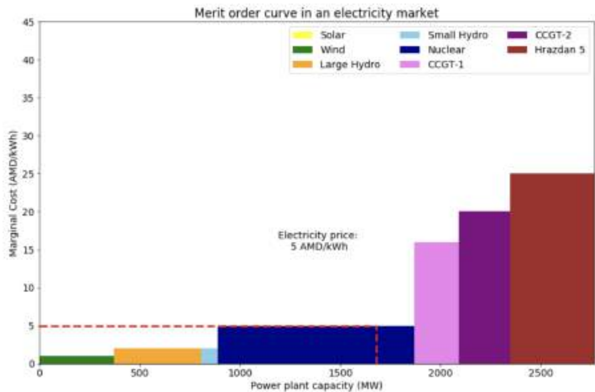
Figure 20. Estimated merit order at peak demand, winter 2040.
