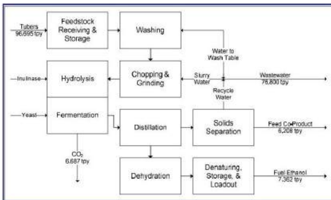
Figure 7. Jerusalem artichoke process plant diagram.
