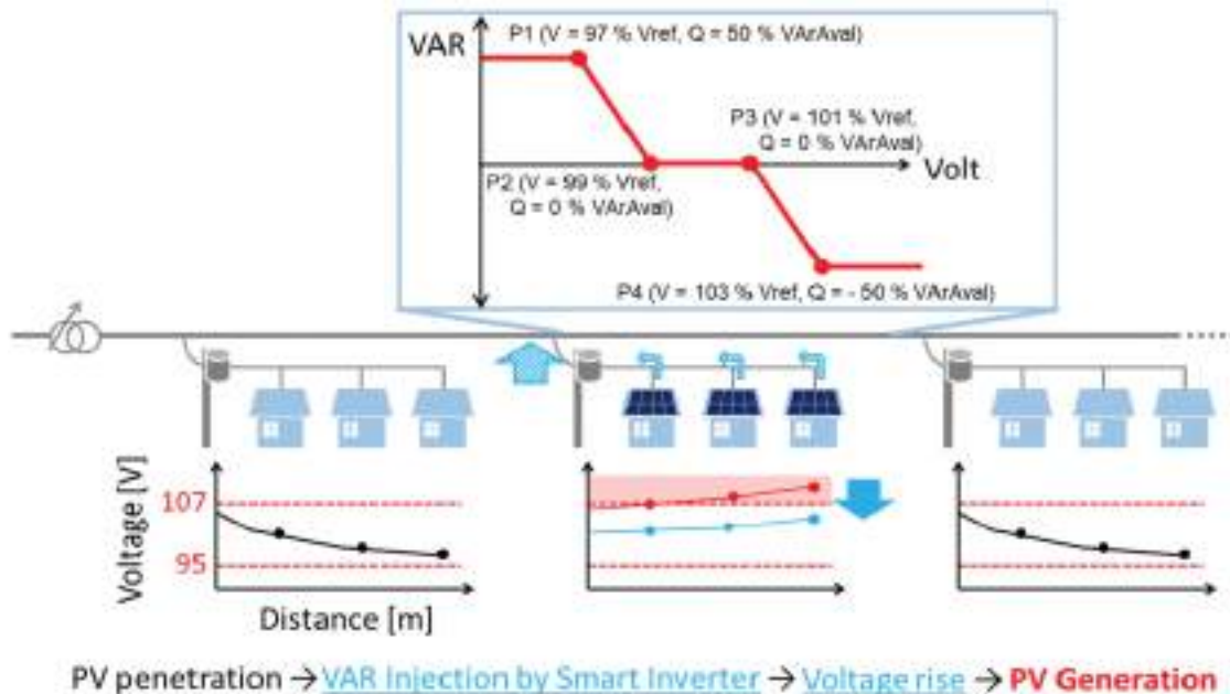
Figure 3. The benefits of smart inverters for distributed generation. Source: Impact of Smart Inverters on Feeder Hosting Capacity of Distribution Networks | IEEE Journals & Magazine
