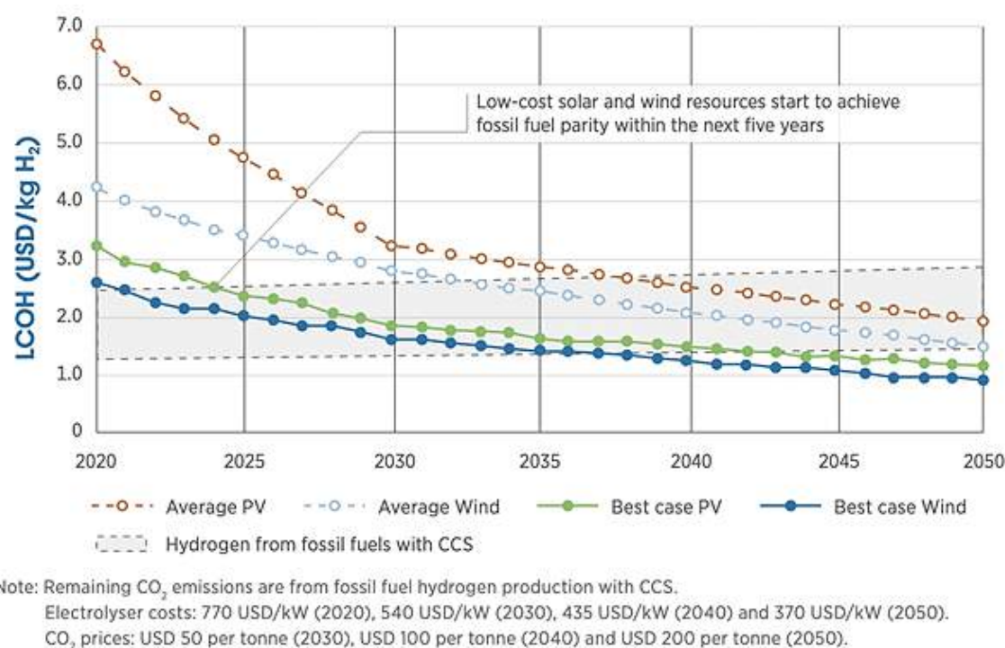
Figure 25. Hydrogen production cost from solar and wind vs. fossil fuels. Source: Hydrogen: A Renewable Energy Perspective (IRENA, 2019).
