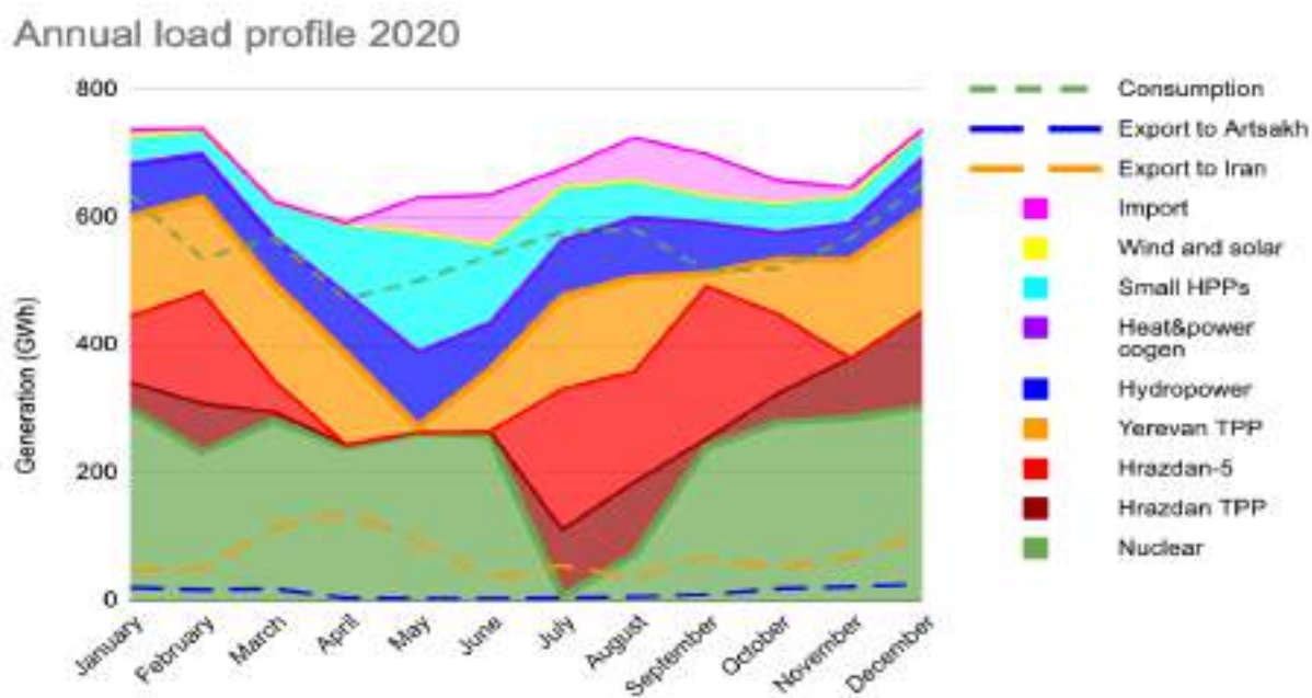
Figure 11. Annual load profile for 2020. Data source: PSRC.am.
