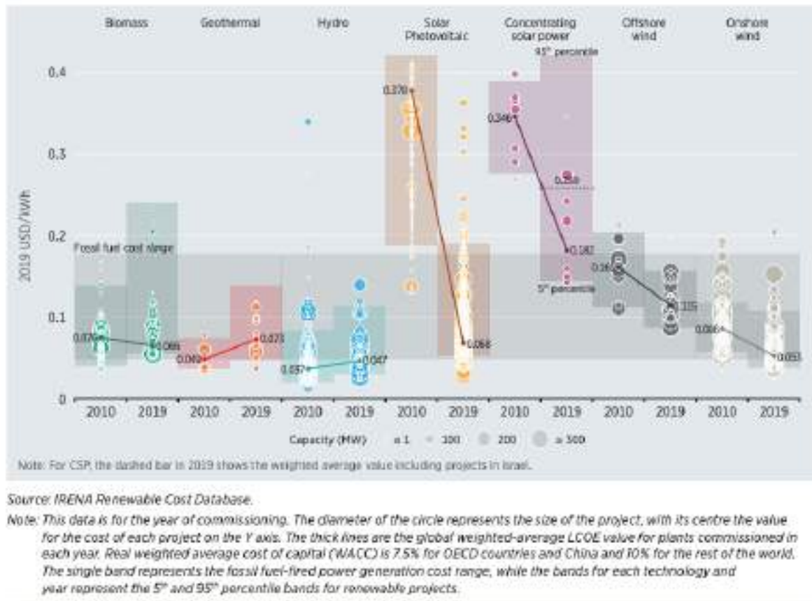
Figure 44. Global LCOEs for different type of renewable energy 54 .
