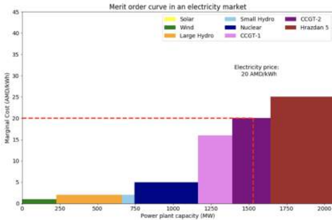
Figure 16. Estimated merit order at peak demand, winter 2035.
