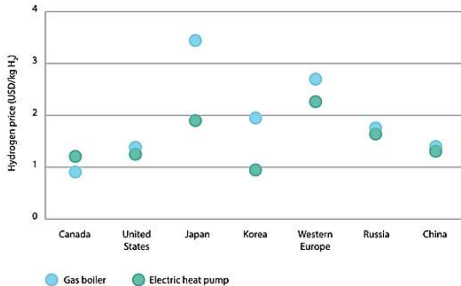
Figure 26. Hydrogen prices needed to become competitive against natural gas boilers and electric heat pumps in selected markets by 2030.
