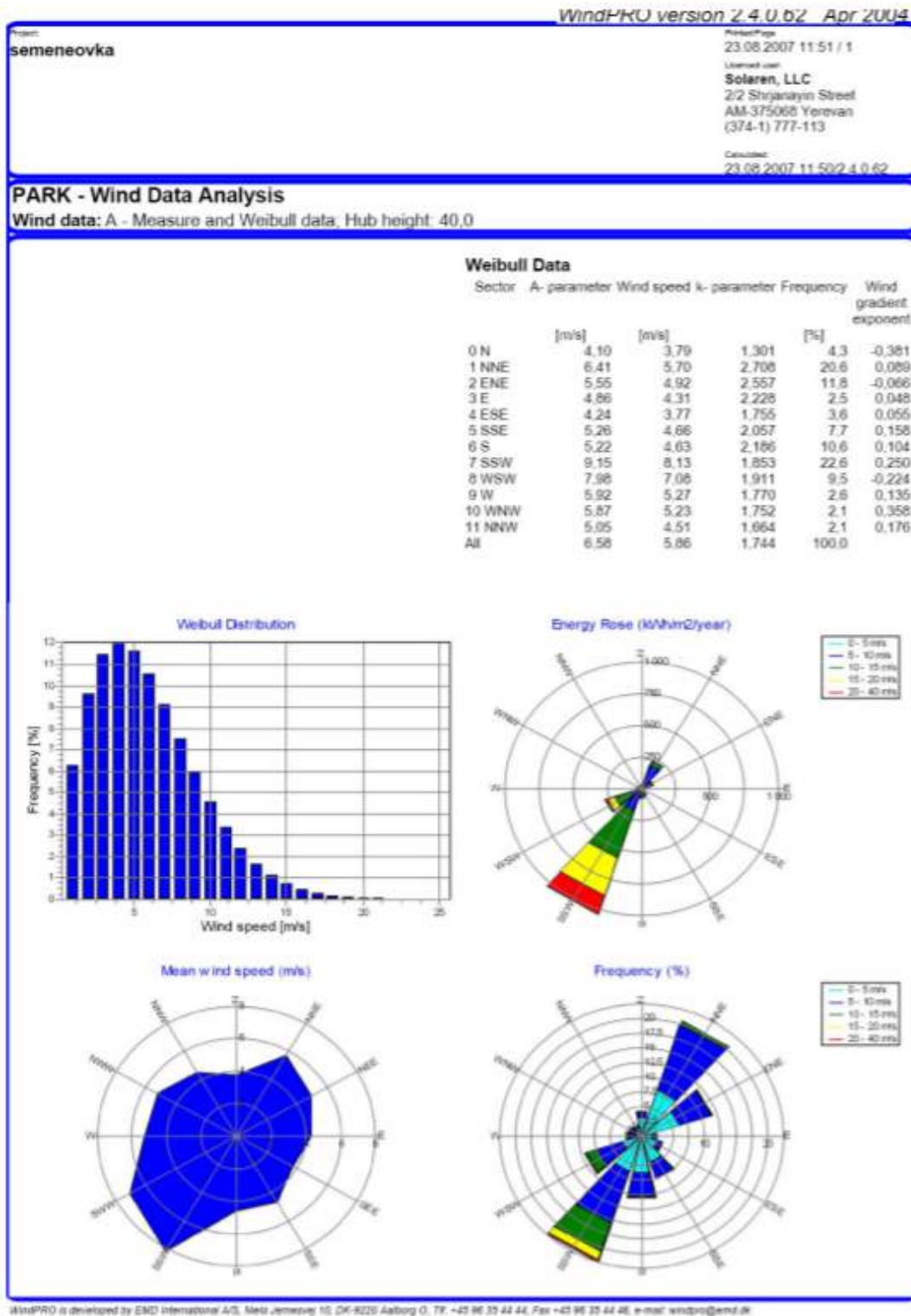
Figure 39. Statistics of the wind distribution for the wind energy project.
