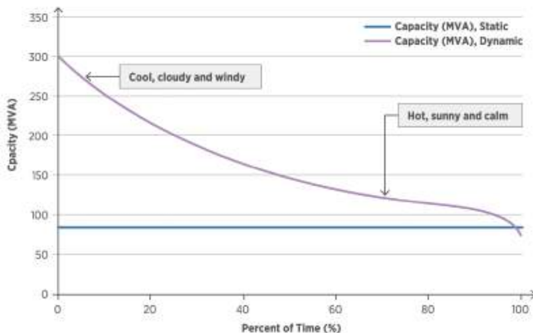
Figure 11. Schematic comparison of static and dynamic current limit.
